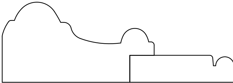
C 5150 - 1-21/32 X 4-3/4 - Backband & bead board sold separately.
