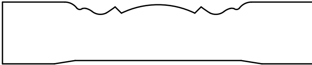
C 4070 - 3/4" x 3-3/4"
