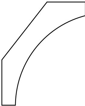
CV 250 - 3/4" x 2-9/16" P=1-5/8" - D=2"
