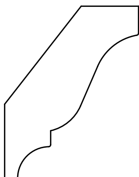
CR 258 - 3/4" x 2-5/8" P=1-5/8" - D=2-1/16"
