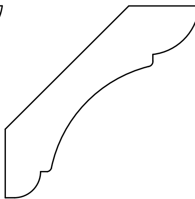
CR 13 - 3/4" x 3-1/4" P=2-5/16" - D=2-5/16"
