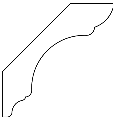
CR 69 - 3/4" x 3-1/4" P=2-5/16" - D=2-5/16"
