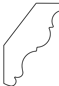
CR 250 - 3/4" x 2-1/4" P=1-5/16" - D=1-27/32"
