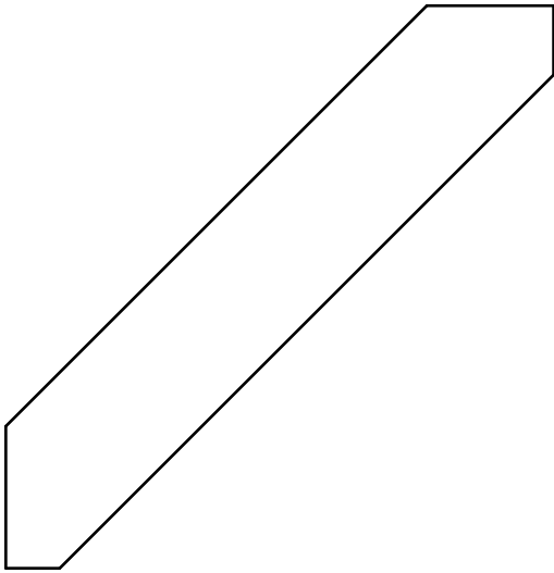
CR 310 - 3/4" x 4-1/4" P=2-31/32" - D=3-1/16"
