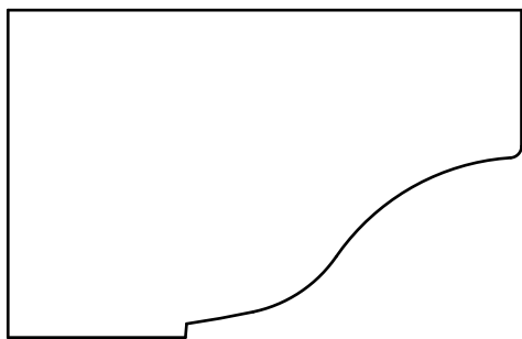
CR 9 - 13/16" x 1-1/2" P=1-1/2" - D=13/16"
