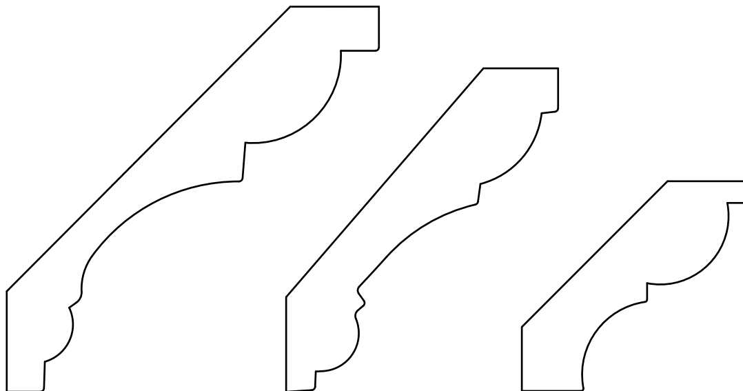
CR 4058 - 13/16'' x 4-9/16'' P= 3-3/16'' - 3-9/32''
