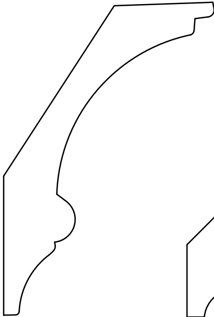
CR 4345 - 1" x 4-11/32" P=2-13/32" - D=3-5/8"
