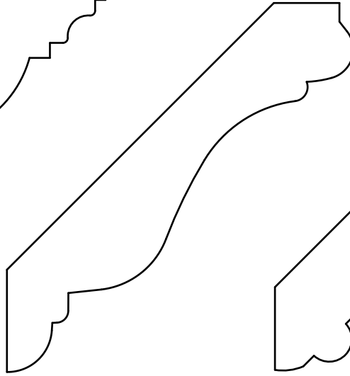
CR 4120 - 13/16" x 4-1/8" P=2-3/4" - D=3-1/16"
