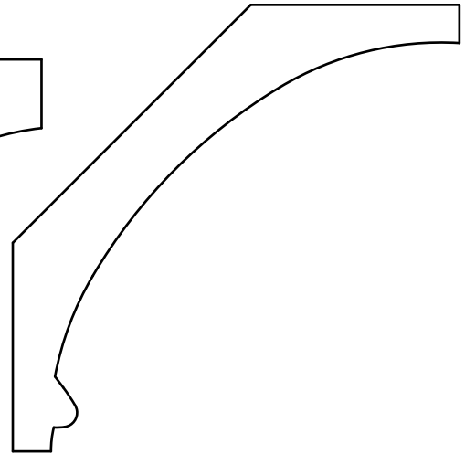
CR 4125 - 1-1/8" x 4-1/16" P=2-7/8" - D=2-7/8"
