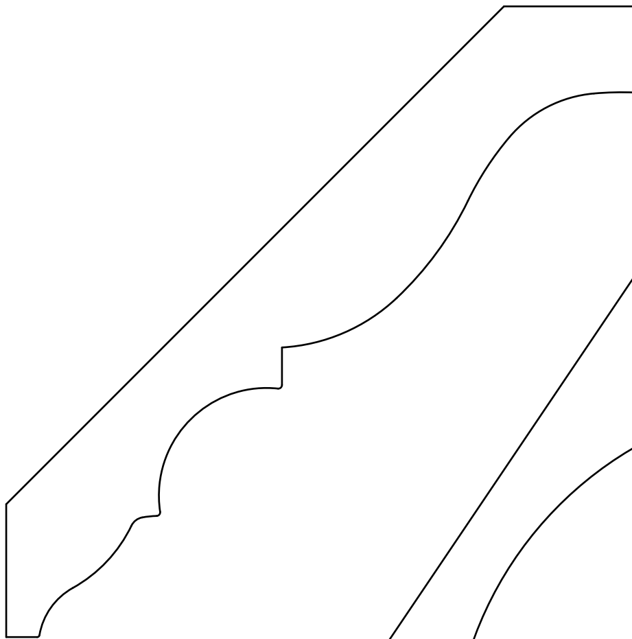
CR 7644 - 1-5/16" X 7-21/32" P=5-3/8" - D=5-3/8"
