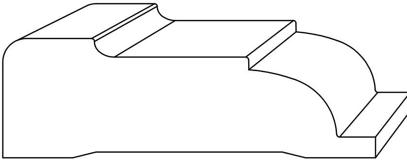
C 4005 - 1-9/32" x 4"
