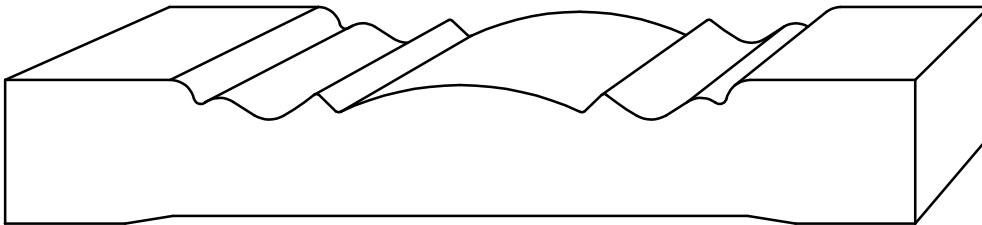
C 4075 - 3/4" x 4-3/4"
