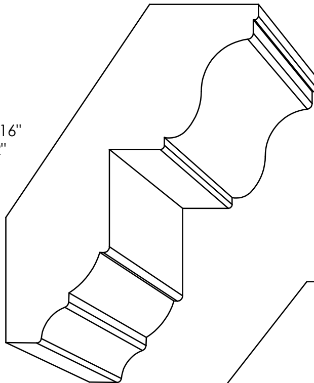
CR 4342 - 1\frac{1}{16}'' \times 4\frac{11}{32}'' P= 2\frac{19}{32}'' - D= 3\frac{1}{2}''
