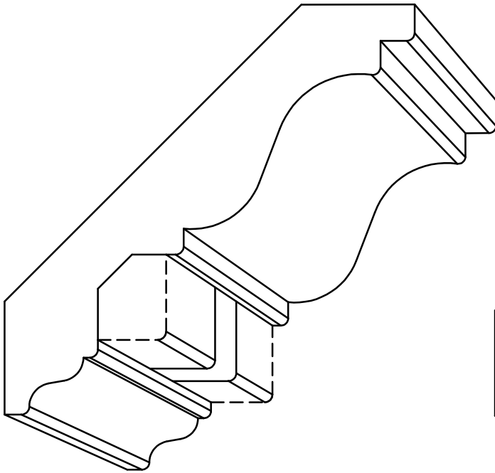
CR 7 - 3/4" x 4-1/4" P=3" - D=3" Pictured with CR 7 Dentil - Sold Separately
