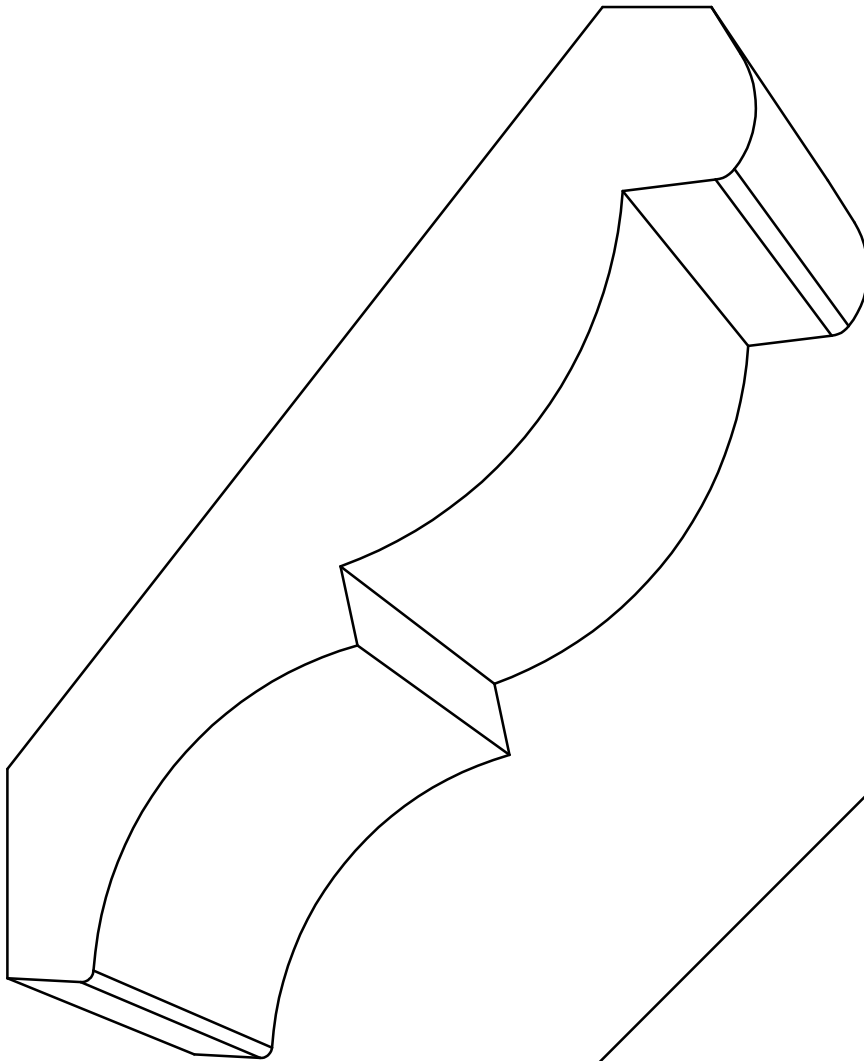
CR 92 - 1-1/16" x 6-1/4" P=3-29/32" - D=5-3/32"
