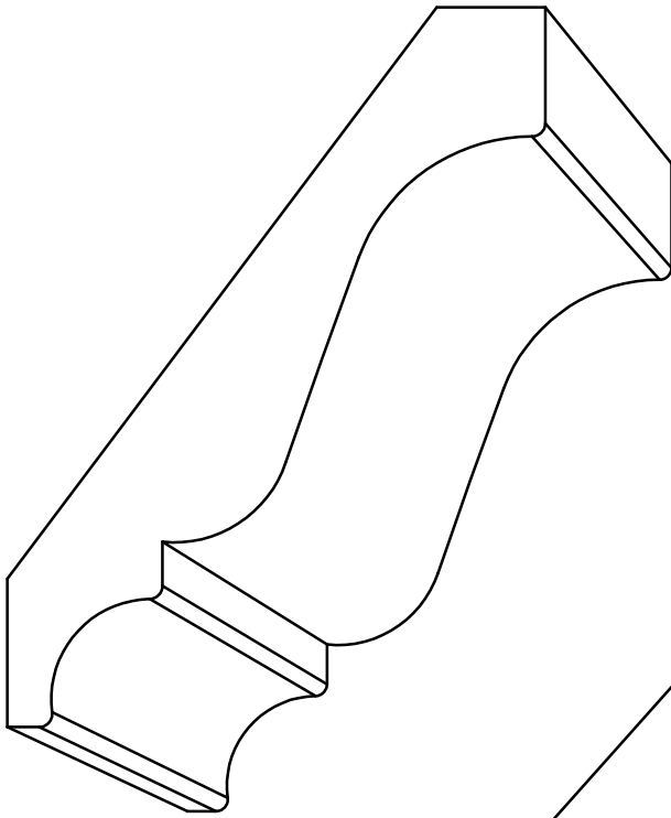
CR 4 - 3/4" x 4-1/4" P=2-17/32" - D=3-13/32"
