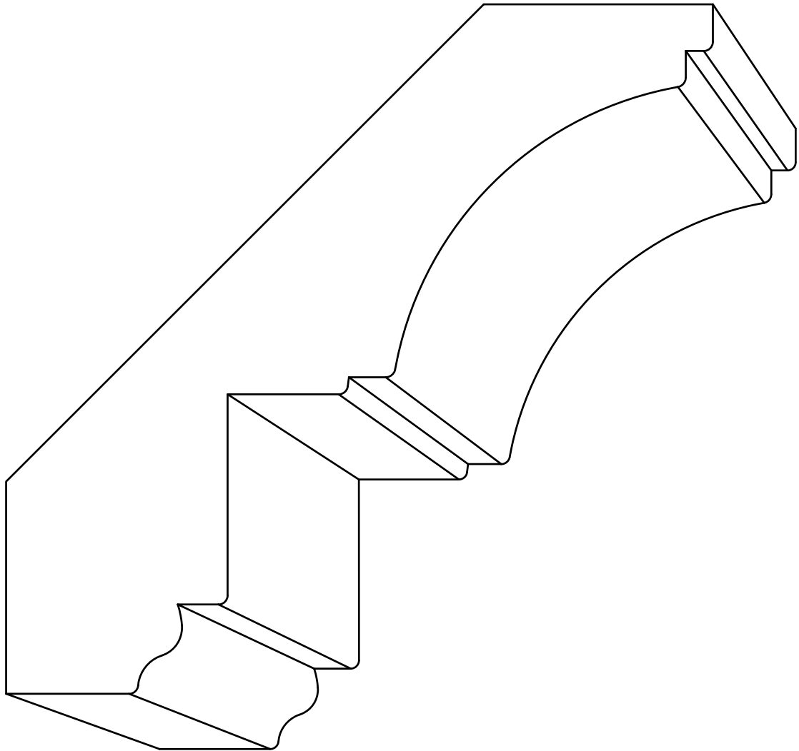
CR 4372 - 1-3/4" x 7-7/32" P=5-5/32" - D=5-1/32"
