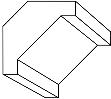
CR 305 - 3/4" x 1-3/4" P=1-1/4" - D=1-1/4"
