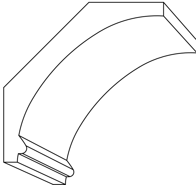
CR 4125 - 1-1/8" x 4-1/16" P=2-7/8" - D=2-7/8"
