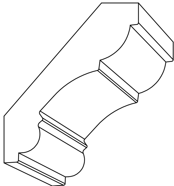
CR 3608 - 3/4" x 3-5/8" P=2-5/16" - D=2-3/4"
