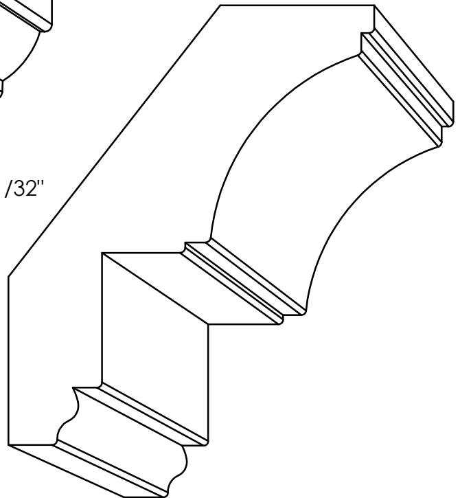
CR 4340 - 1\frac{1}{16}'' \times 4\frac{11}{32}'' P= 2\frac{25}{32}'' - D= 3\frac{11}{32}''
