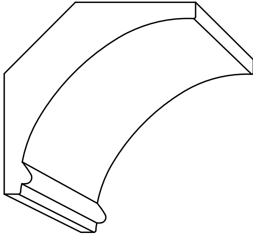
CR 4124 - 1" x 2-13/16" P=2" - D=2"
