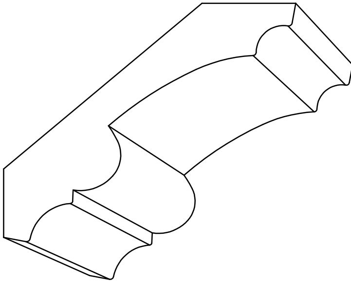
CR 3078 - 13/16" x 4" P=3-1/8" - D=2-1/2"
