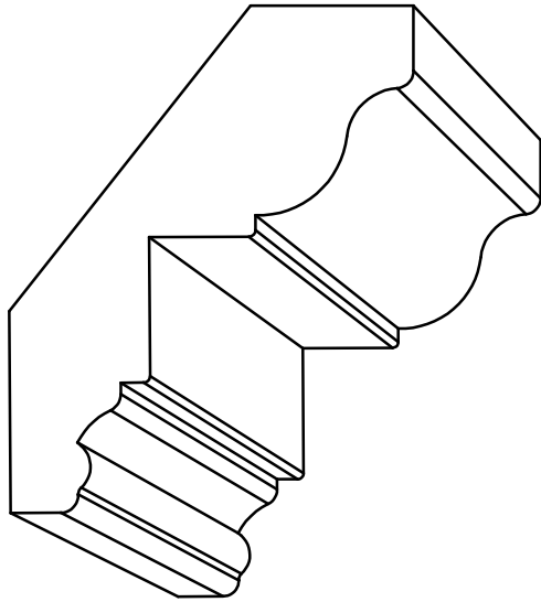
CR 3340 - 1\frac{3}{16}'' \times 3\frac{1}{16}'' P= 1\frac{29}{32}'' - D= 2\frac{13}{32}''
