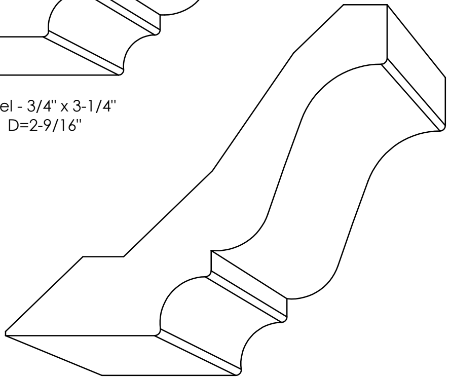
CR 4 w/ Heel - 3/4" x 4-1/4" P=2-21/32" - D=3-13/32"
