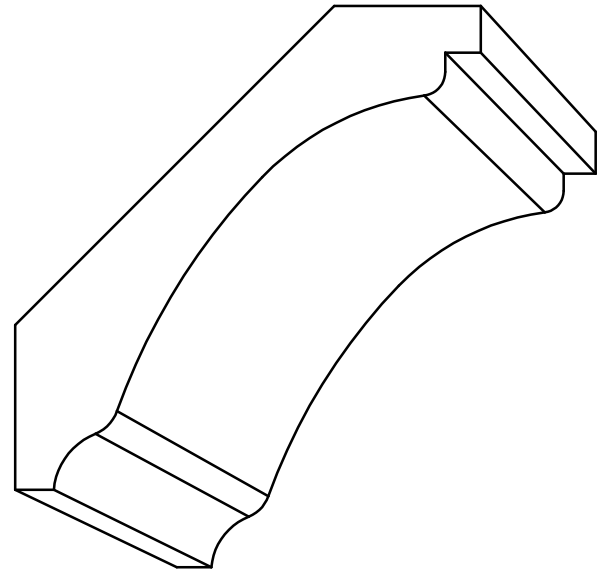
CR 3074 - 3/4'' \times 3-1/2'' P= 2-7/16'' - D= 2-17/32''
