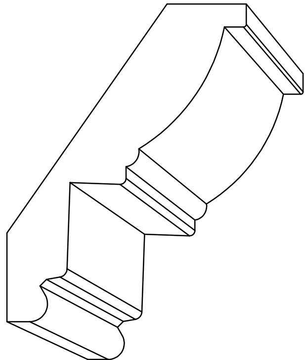
CR 4562 - 13/16" x 4-3/16" P=2-17/32" - D=3-11/32"
