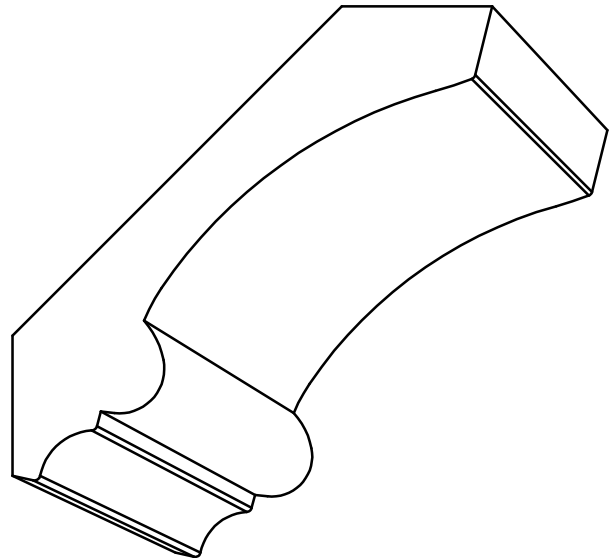
CR 3076 - 3/4" x 3-1/2" P=2-1/2" - D=2-15/32"
