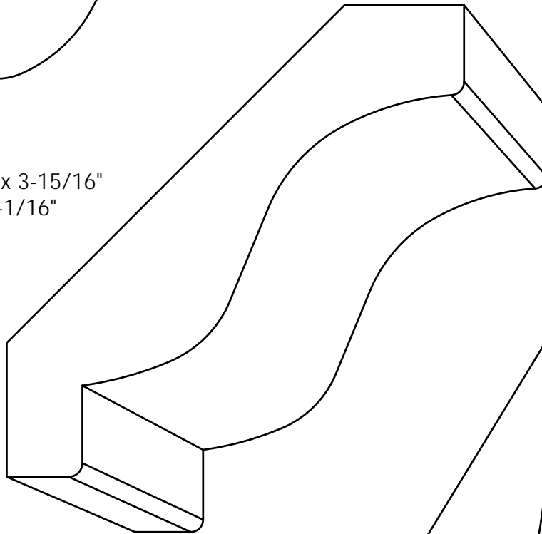
CR 2386 - 1" x 4\frac{13}{16} " P= 3\frac{5}{16} " - D= 4\frac{7}{16} "
