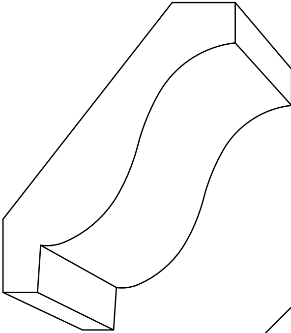
CR 2380 - 1\frac{3}{16} " x 3\frac{15}{16} " P= 2\frac{15}{32} " - D= 3\frac{1}{16} "
