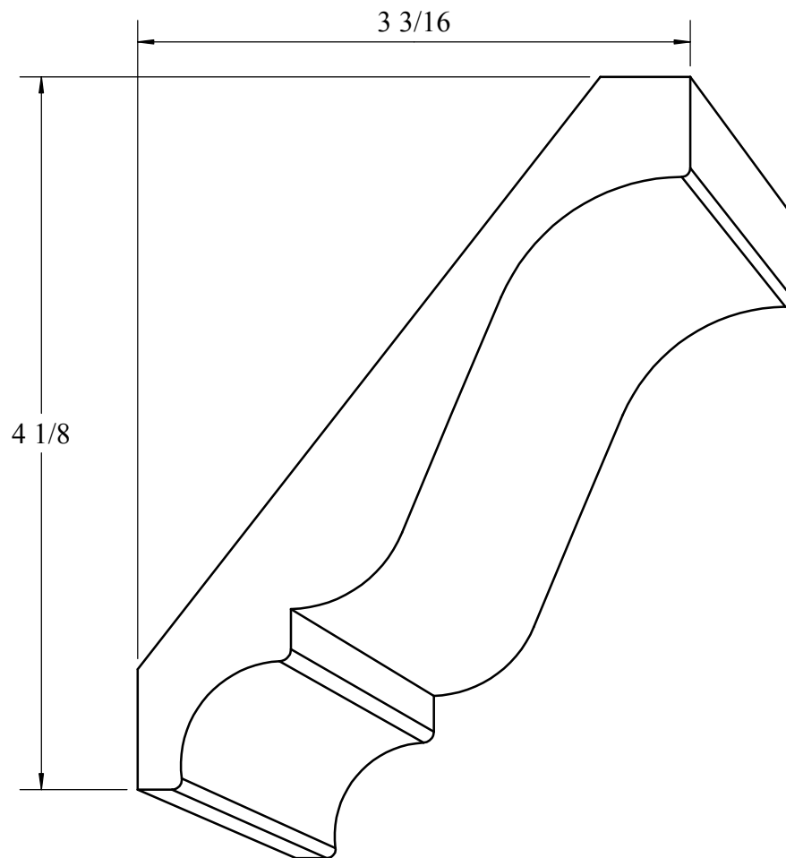
CR 5 - \frac{3}{4} " x 5\text{-}\frac{1}{4} " P= 3\text{-}\frac{3}{16} " - D= 4\text{-}\frac{1}{8} "
