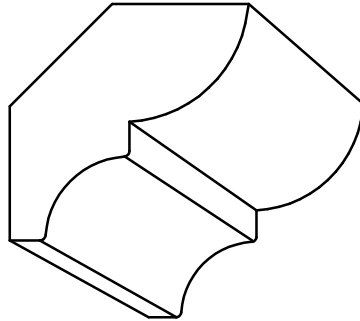
CR 10 - 5/8" x 1-3/4" P=1-1/4" - D=1-7/32"
