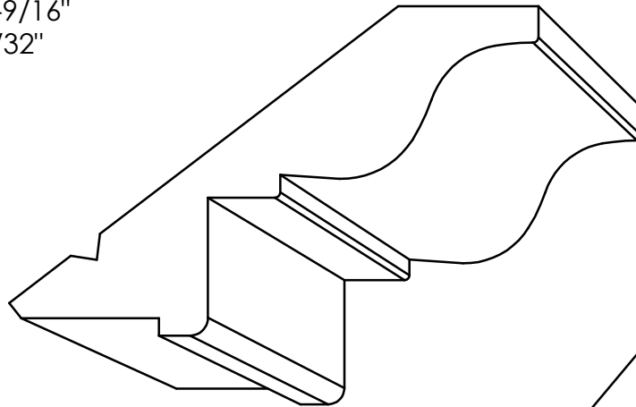
CR 4550 - 1\frac{3}{16} " x 3\frac{1}{2} " P= 2\frac{7}{32} " - D= 1\frac{13}{16} "
