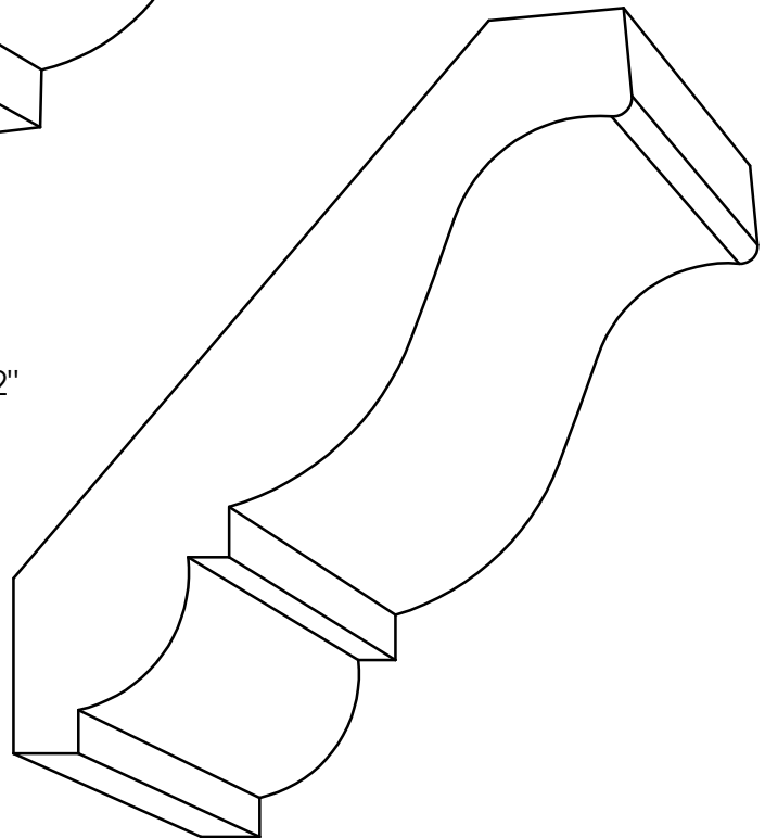
CR 3627 - 25/32" x 4-5/8" P=2-15/16" - D=3-19/32"
