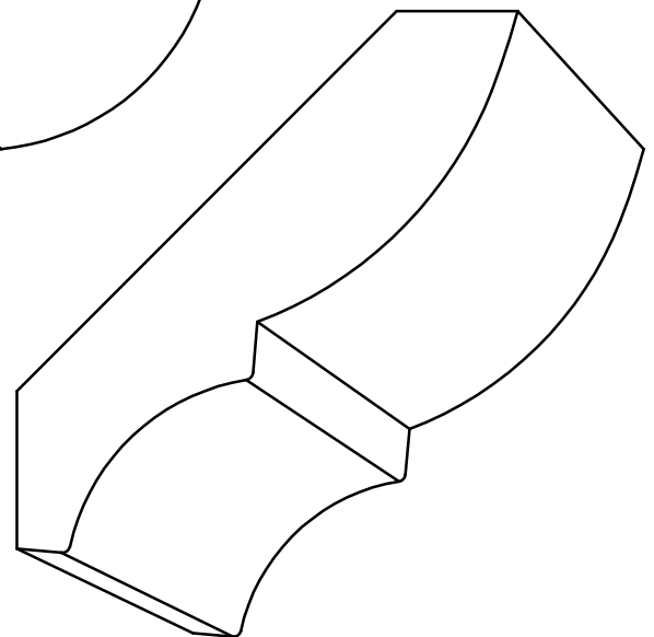
CR 350 - 3/4" x 3-1/2" P=2-3/8" - D=2-9/16"
