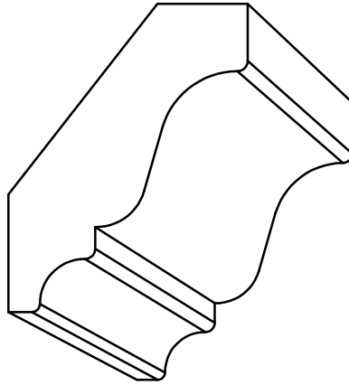
CR 2 - 5/8" x 2-1/4" P=1-3/8" - D=1-25/32"
