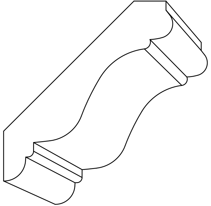
CR 4120 - 13/16" x 4-1/8" P=2-3/4" - D=3-1/16"
