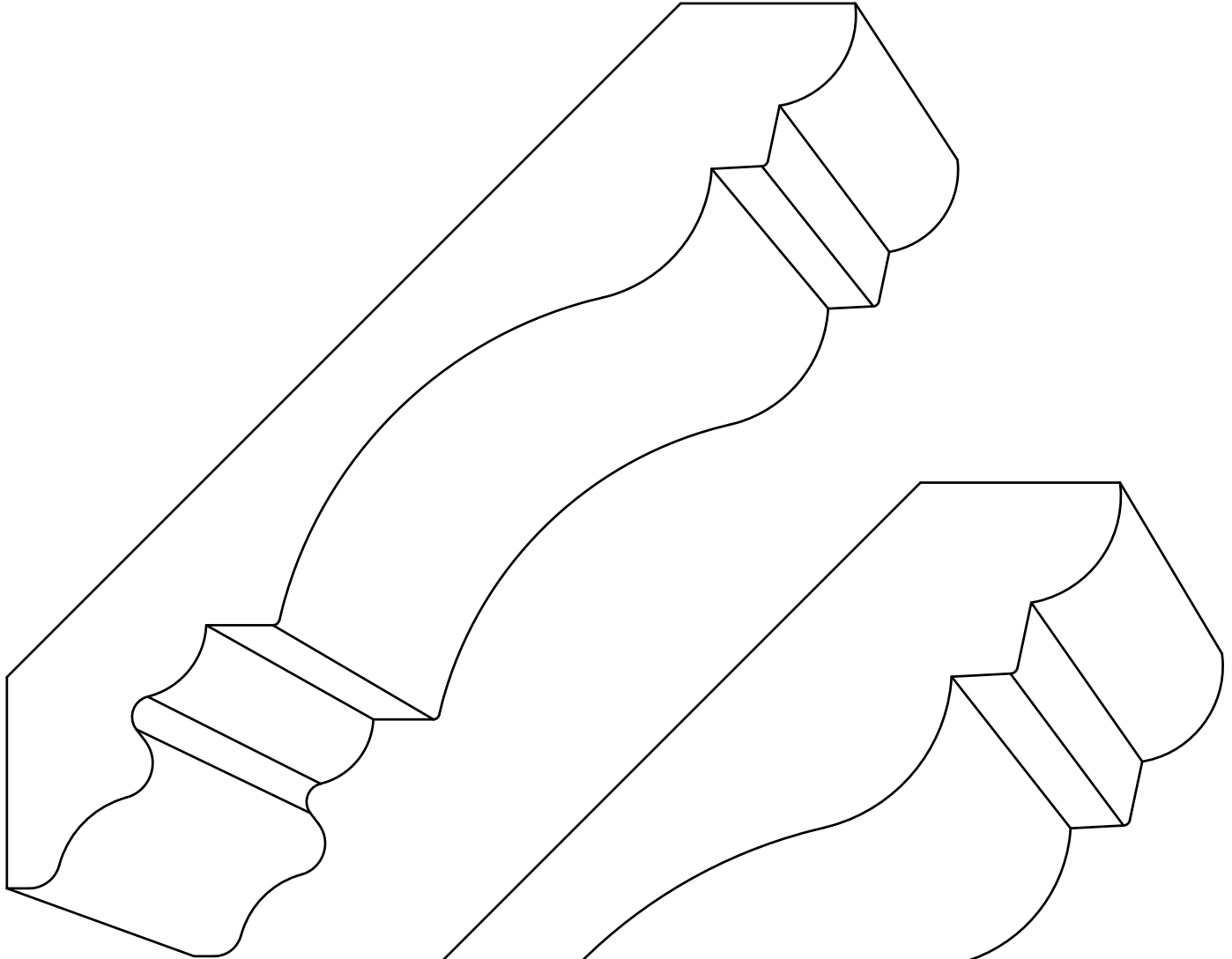
CR 7518 - 1-1/32" x 7-1/4" P=5" - D=5-1/4"
